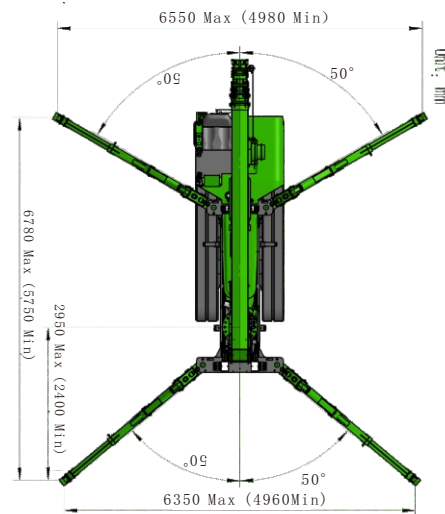
Outrigger Footprints
